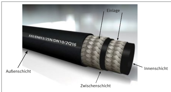
Abb. 1 Hydraulik-Schlauch
